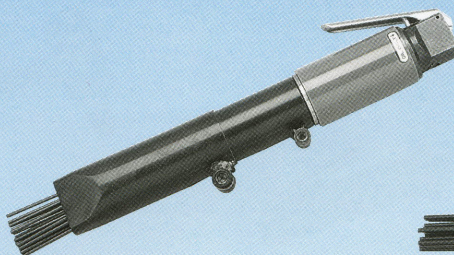
PT2823 straight type Needle: \varnothing 3mm \times 19pcs
