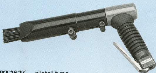
PT2826 pistol type Needle: \varnothing 3mm \times 19pcs
