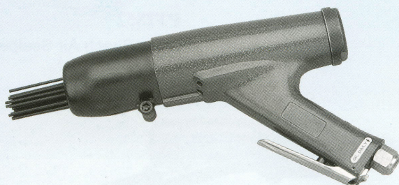
PT28153 industrial model Needle: \varnothing 3mm \times 28pcs
