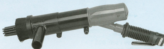
PT2321 Needle Scaler attachment - round shank PT2321H Needle Scaler attachment - hex. shank
