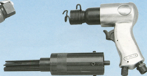
PT282 pistol type Needle: \varnothing 3mm \times 19pcs
